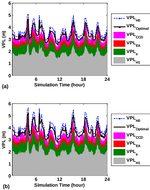
Figure 6. VPLs of LAD-GNSS for (a) UAV operating in Coverage I, and (b) UAV operating in Coverage II
