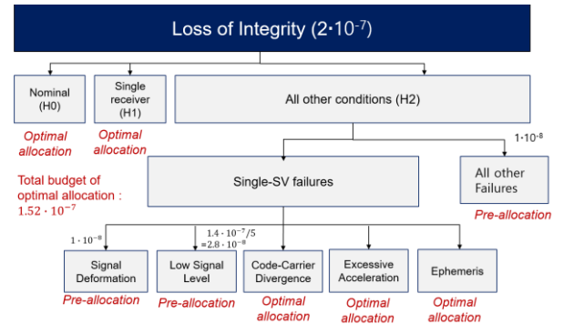
Figure 4. Integrity risk allocation of LAD-GNSS for UAV
